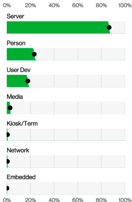
Figure 19. Assets in breaches (n=4,433)
