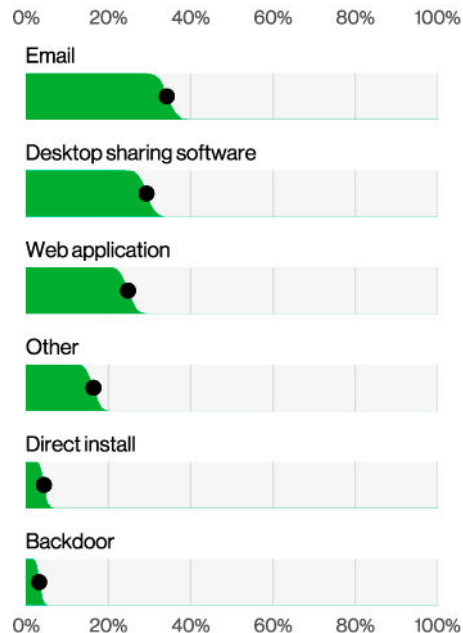
Figure 31. Action vectors for Ransomware (n=690)
